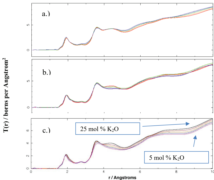
FIGURE 4. Total correlation functions from x-ray diffraction analysis: (a) \text{Li}_2\text{O}-\text{TeO}_2 , (b) \text{Na}_2\text{O}-\text{TeO}_2 , and (c) \text{K}_2\text{O}-\text{TeO}_2 . The following was observed: Short Te–O bonds (1.85–1.88 Å) and a longer Te–O bond and O–O bond at (2.5–2.9 Å). The different colored lines represent the various mol % of alkali oxide in the glass. The alkali content increases such that 5 mol % of alkali oxides is the bottom line and 25 mol % is the top line, as shown in Fig. 4c.
