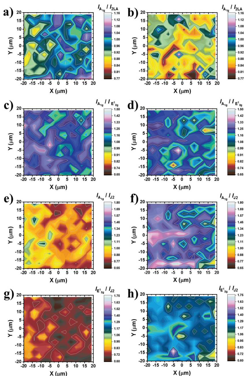
Fig. 3 Raman intensity ratio maps from a 20\ \mu\text{m} \times 20\ \mu\text{m} area (3 nm step, 196 points per spectra) of ce - \text{MoS}_2 and B15C5-MoS 2 . (a, b) Plots of A_{1g}/2L_A for ce - \text{MoS}_2 and B15C5-MoS 2 , respectively. (c, d) Plots of A_{1g}/E_{2g}^1 for ce - \text{MoS}_2 and B15C5-MoS 2 , respectively. (e, f) Plots of A_{1g}/J_2 for ce - \text{MoS}_2 and B15C5-MoS 2 , respectively. (g, h) Plots of E_{2g}^1/J_2 for ce - \text{MoS}_2 and B15C5-MoS 2 , respectively. All spectra recorded under on-resonance excitation (633 nm, 0.3\ \text{mW cm}^{-2} ) under ambient conditions. A projection of each map is also given at the bottom for clarity. The spectra acquired for constructing the maps are presented in the ESI, Fig. S7.†
