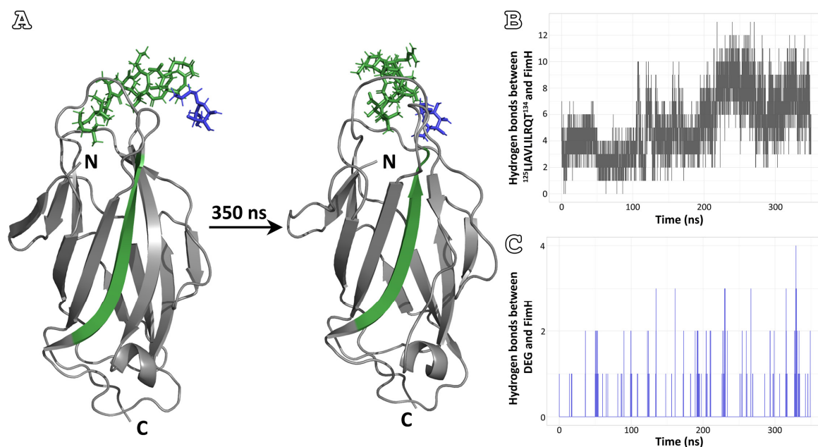
Figure 4. MD simulations of lectin domain-DEG- ^{125}\text{LIAVLILRQT}^{134} complex. (A) First (0 ns, left) and last (350 ns, right) frames of MD simulations. ^{125}\text{LIAVLILRQT}^{134} peptide-analogue is colored green, and DEG is colored blue (N: N-terminal, C: C-terminal). (B) The number of hydrogen bonds formed between ^{125}\text{LIAVLILRQT}^{134} peptide-analogue and FimH lectin domain. More bonds are formed by the end of the simulation. (C) The number of hydrogen bonds formed DEG and FimH lectin domain. The number of hydrogen bonds between the two molecules fluctuates during the simulation, with that being zero in most instances.
